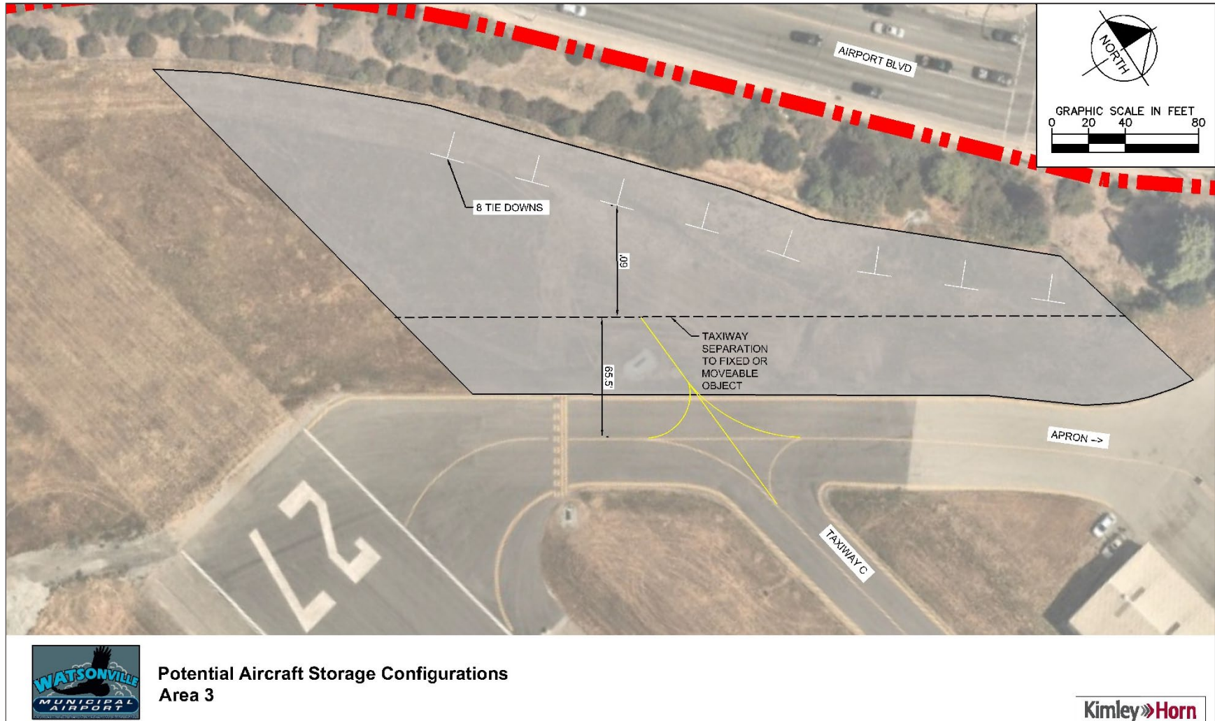
Figure 4-24: Aircraft Storage Area 3 - Potential Configuration
